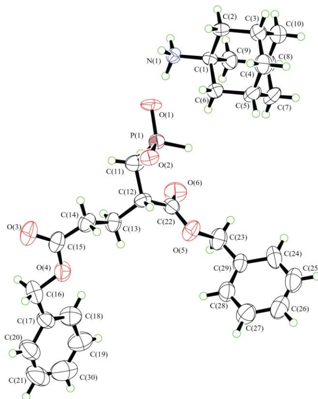
Figure 2. Crystal structure of ( S )-(-)-4-1-adamantanamine salt.
